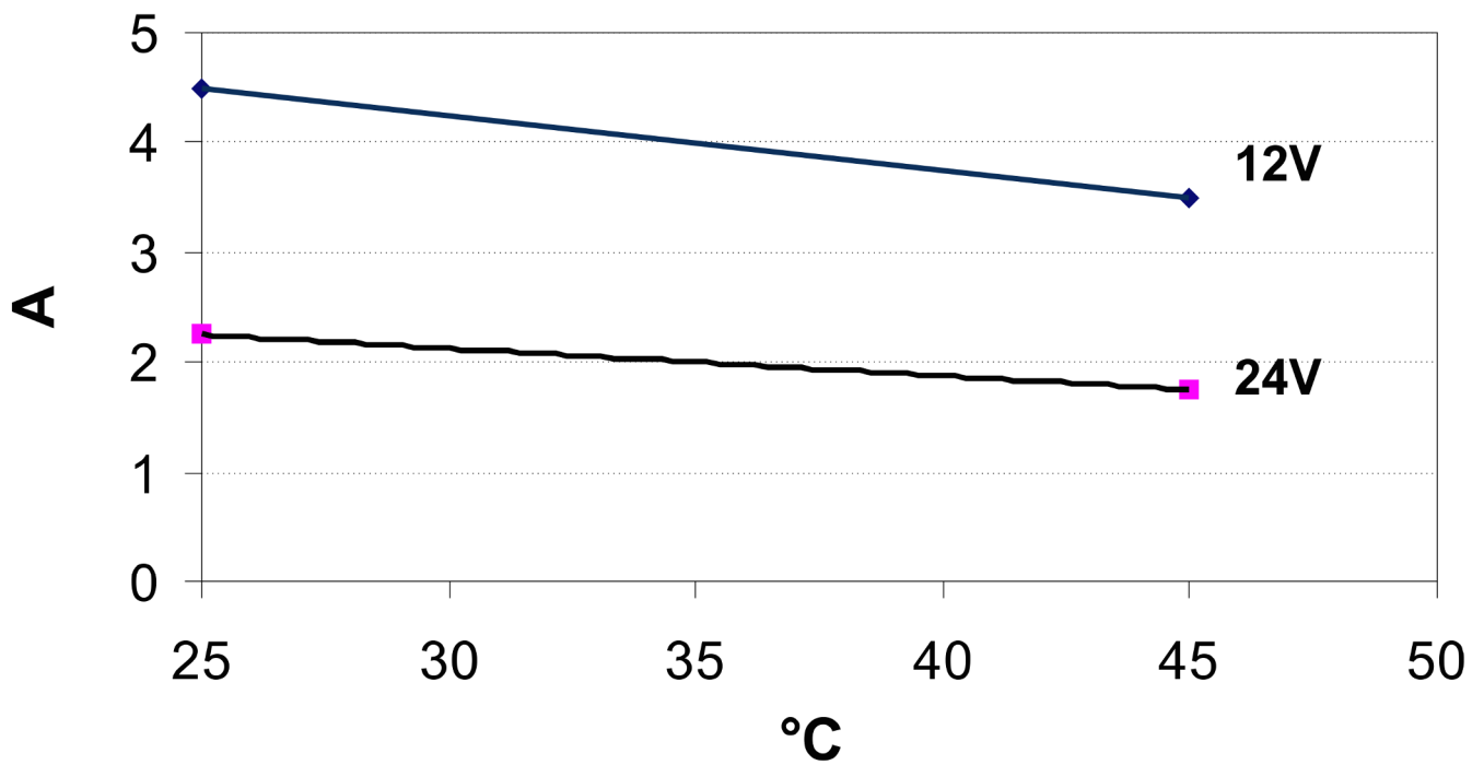
DIAGRAMMA ASSORBIMENTI AMPERE-DRAW DIAGRAM
